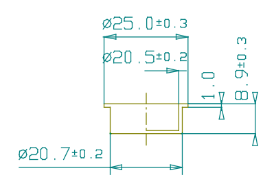
27ネジポリ中栓
